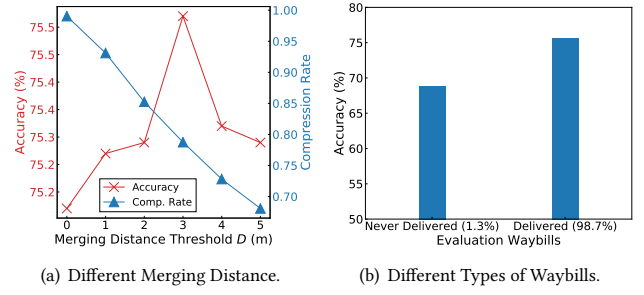
Figure 11: Effectiveness Experiments.
