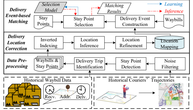
Figure 4: System Framework.
