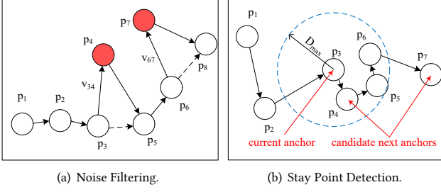
Figure 5: Trajectory Pre-processing.
